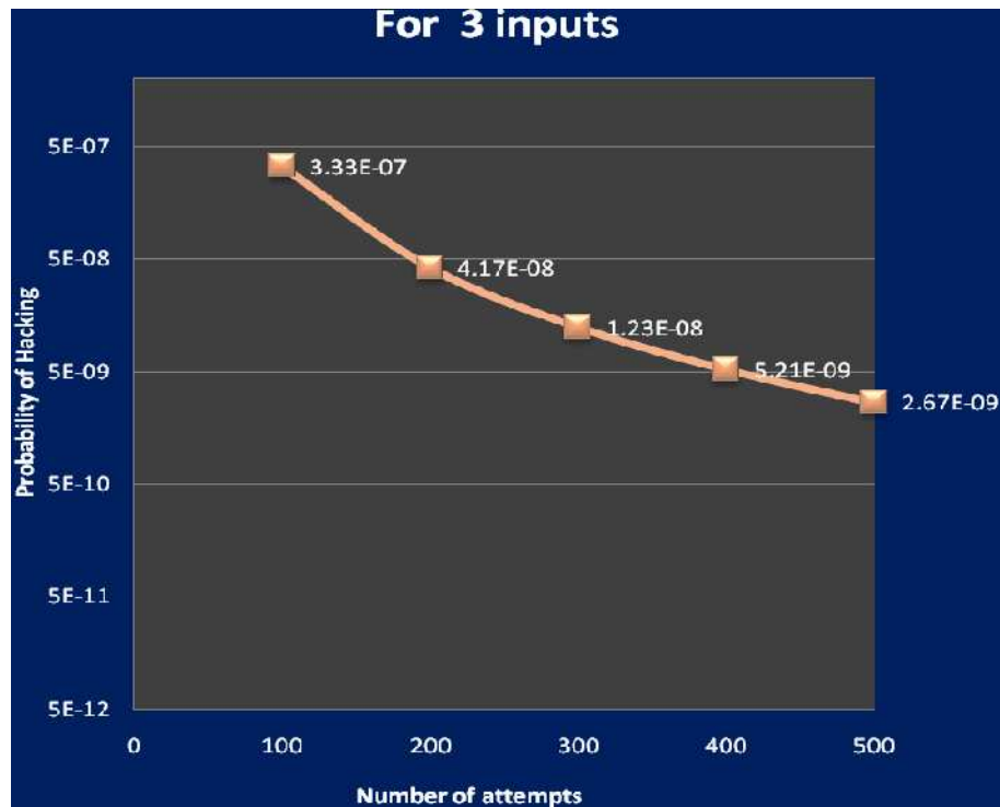
Fig 8: shown the probability of hacking for given number of attempts
